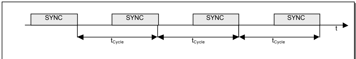
Figure 10: Communication Cycle Period
