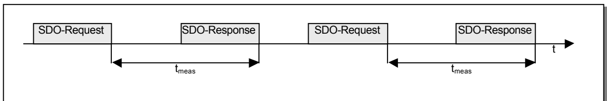
Figure 5: SDO Response Time
