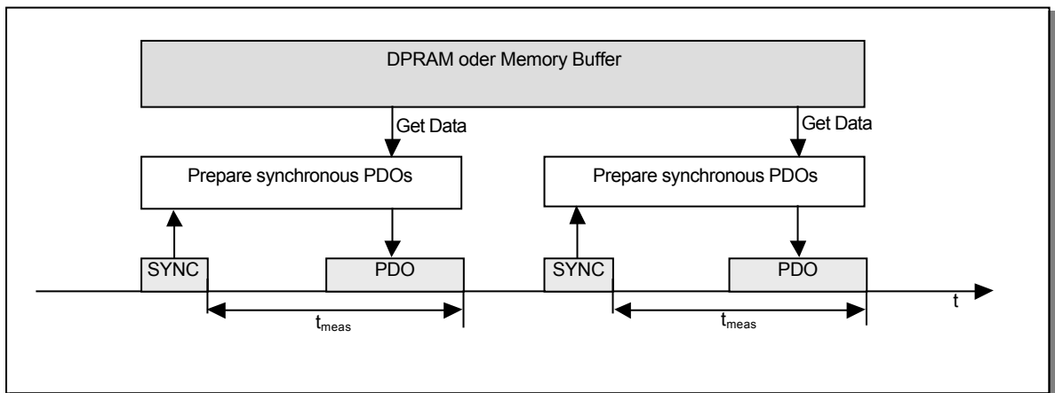
Figure 4: SYNC Reaction Time
