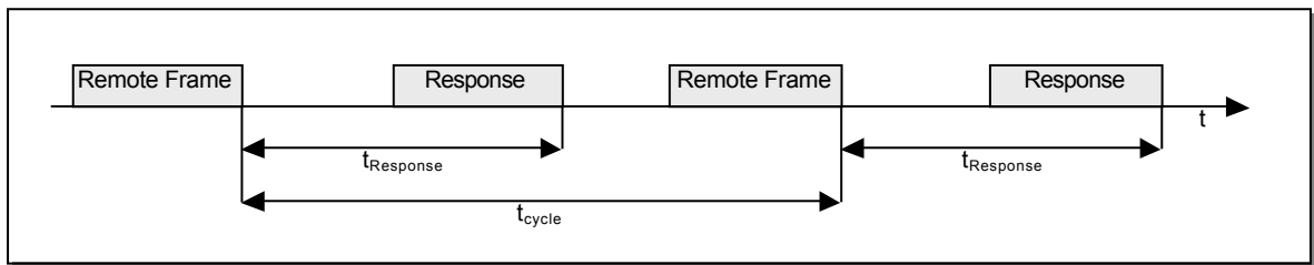
Figure 7: Guard Response Time and Guard Cycle Time
