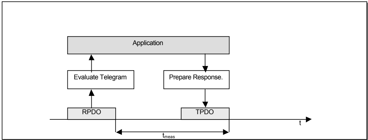
Figure 3: PDO Turnaround Time
