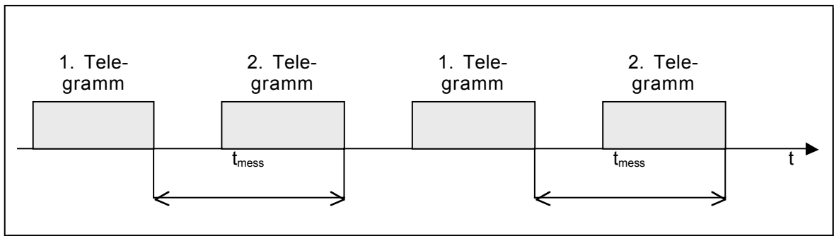
Figure 2: Reaction time measurement
