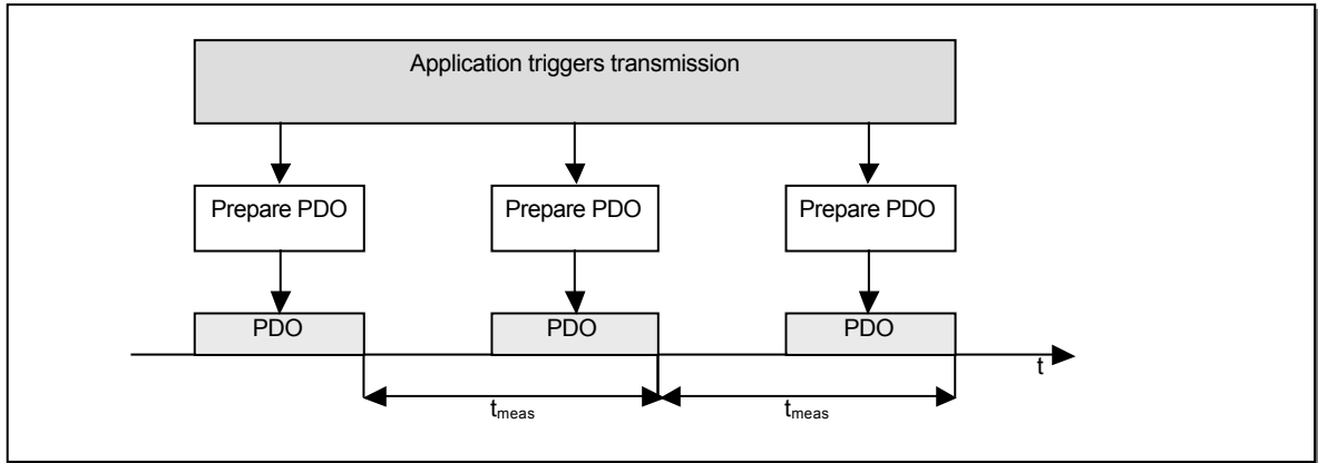
Figure 9: PDO Timer Event Cycle Time
